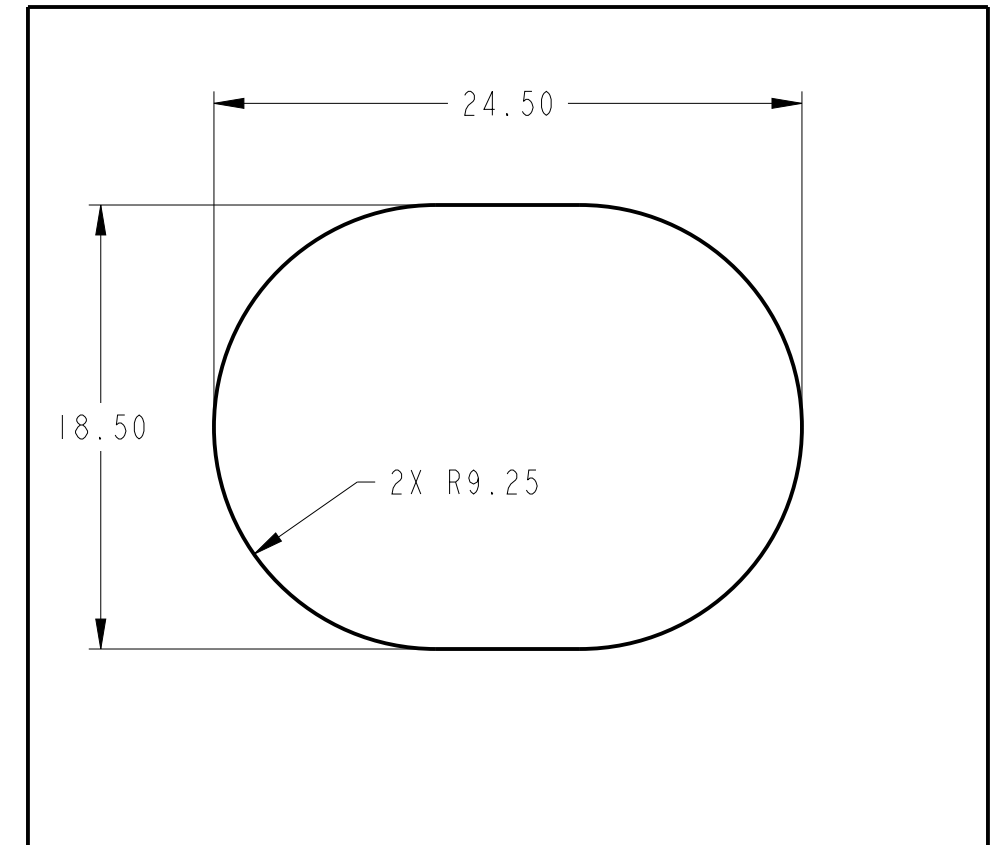
CUTOUT DIMENSION VIEW SCALE 1:8
