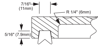
GASKET GROOVE, SECTION B:B
